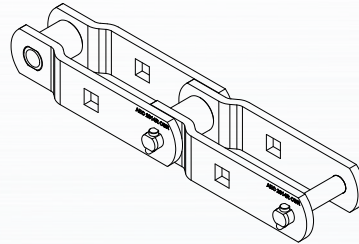
Figure 2-4. Cranked-plates rollerless chain for outboard rollers
