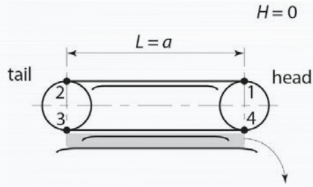
Figure 2-16. Horizontal drag conveyor working under load
