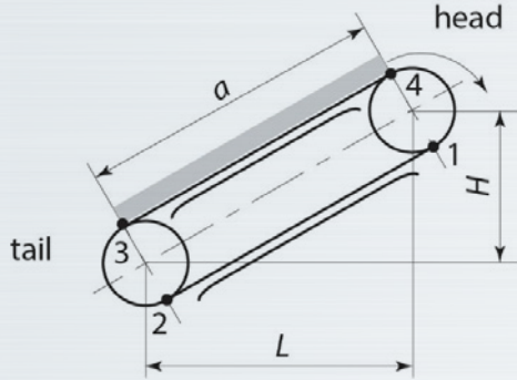
Figure 2-15. Inclined apron conveyor working under load
